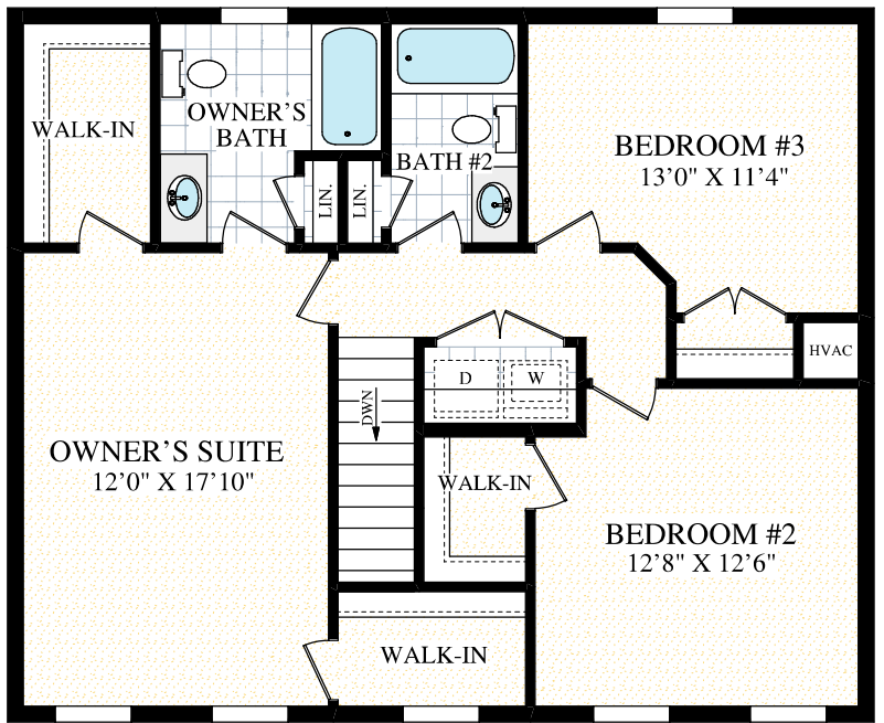
2ND FLOOR LEVEL
